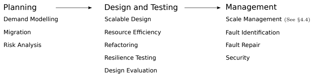
Figure 5: An Overview of the Software Engineering Tasks facing Cloud Providers and their Clients that may be amenable to an SBSE Approach
